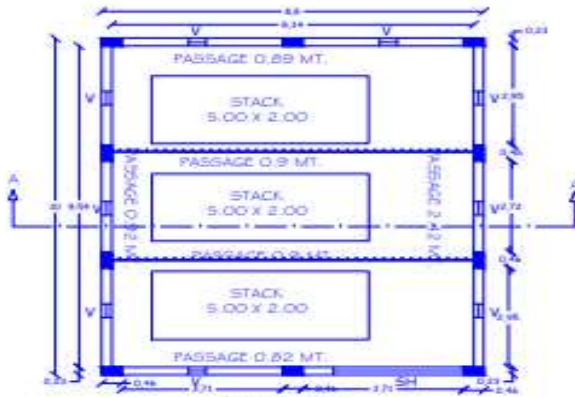
GODOWN PLAN SCALE 1:100
